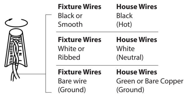
Fig.2 Wiring
